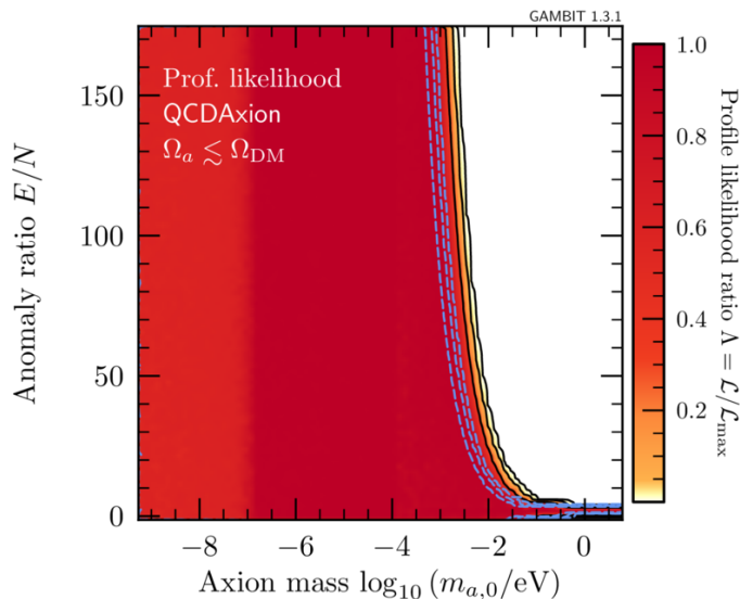
Figure 1. Example for the effect of wrongly defining the axion-photon coupling. The colour map and black lines are for the corrected figure using GAMBIT 1.3.1, while dashed blue lines indicate the previous erroneous exclusion lines from GAMBIT 1.3.0.
