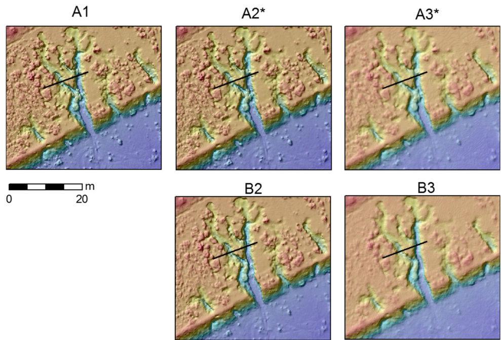
Fig. 7 Subsets showing the DSMs of a terraced abandoned agricultural field that is incised by different gully systems. The blue and red color represent 469 - 473 m elevation. The black lines show the location of the cross section presented in Fig. 8. The outline of the subset is highlighted by the blue rectangle in Fig. 4
