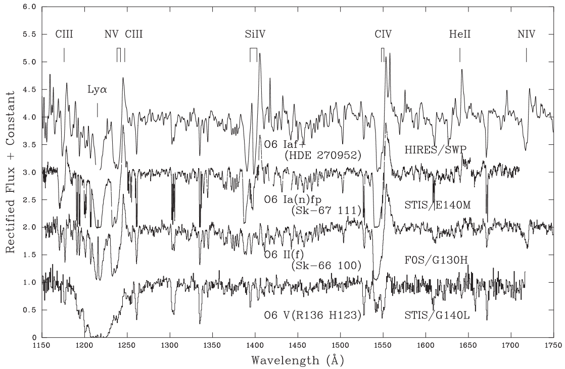
Figure A9. Montage of O6 luminosity sequence. C IV \lambda\lambda 1548\text{--}51 and N V \lambda\lambda 1238\text{--}42 exhibit a weak P Cygni profile for dwarfs, in contrast to strong P Cygni profiles at class II–I, with Si IV \lambda\lambda 1393\text{--}1402 also exhibiting saturated P Cygni profiles for supergiants. Narrow He II 1640 emission is also observed in supergiants.
