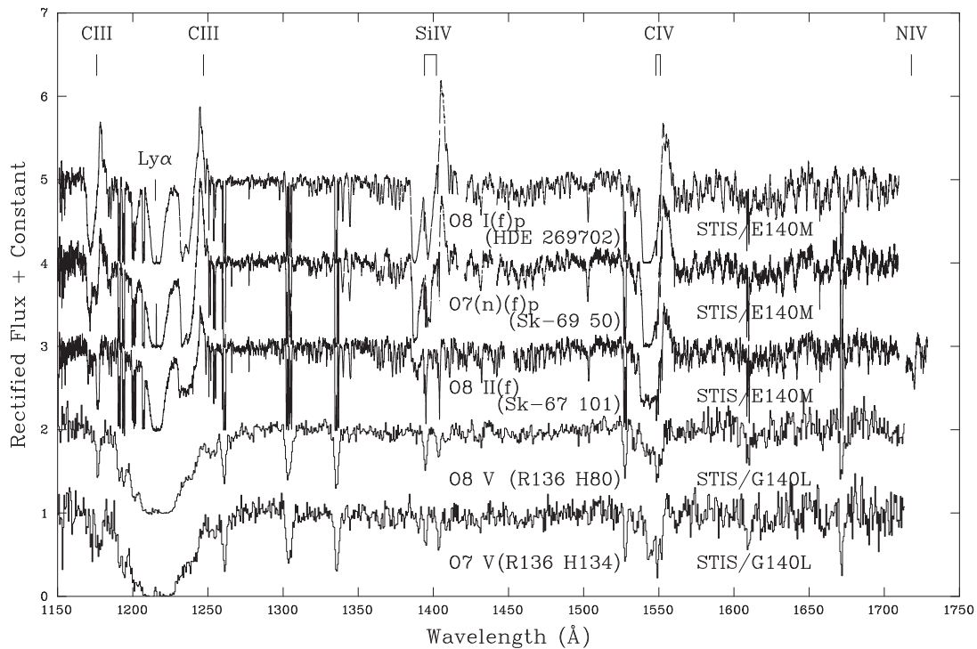
Figure A10. Montage of O7–8 luminosity sequence. C IV \lambda\lambda 1548\text{--}51 exhibits a narrow, weak P Cygni profile for dwarfs, with N V \lambda\lambda 1238\text{--}42 barely present. Both lines display a prominent P Cygni profile at Class II (unsaturated for N V), while Si IV \lambda\lambda 1393\text{--}1402 exhibit saturated P Cygni profiles amongst supergiants.
