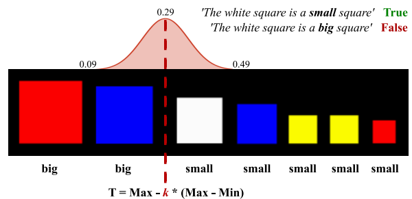
Figure 1: Our approach: given a visual context depicting several objects and a sentence about one object size, models have to assess whether the sentence is true or false. Ground-truth answers are context -specific and depend on a threshold T (Schmidt et al., 2009) which counts objects as ‘big’ based on: (1) the area of the biggest (Max) and smallest (Min) object in the context; (2) the value of a ‘vague’ k determining the top k\% of sizes which count as ‘big’. In our approach, all objects that are not ‘big’ count as ‘small’. Best viewed in color.
