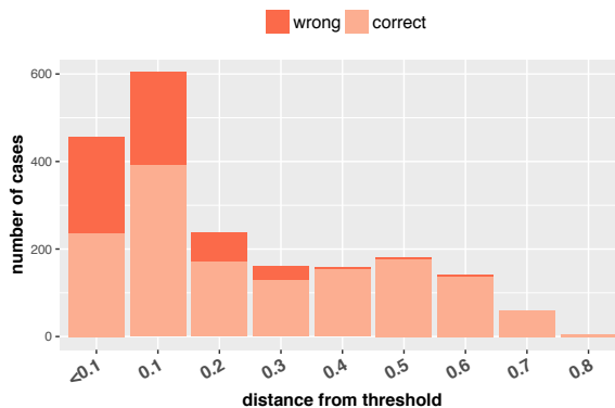
Figure 6: SET+POS-hard . Correct and wrong predictions by best run of FiLM (73% acc.) against distance from the threshold. Best viewed in color.
