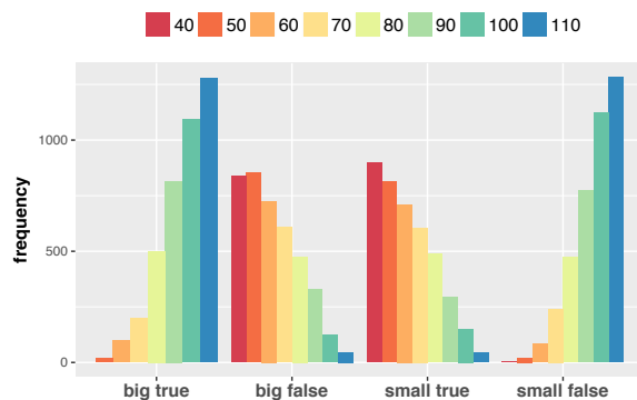
Figure 3: POS . Distribution of queried objects’ areas per question type in train. This plot highlights an important feature of MAlLeViC, namely that objects with any area from 40 to 110 can be either ‘big’ or ‘small’ depending on the visual context. Best viewed in color.
