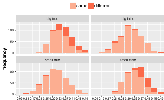
Figure 5: SET+POS-hard . Distribution of k against sentence type (clockwise from top-left: big true, big false, small false, small true). Cases labelled as different are those for which the ground truth adjective (e.g. ‘big’) would change with k = 0.29 (e.g., ‘small’); in same cases, it would be the same. Best viewed in color.
