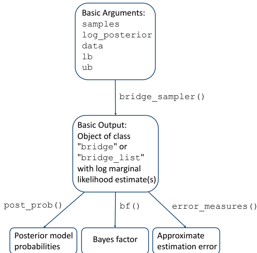
Figure 1: Flow chart of the steps that a user may take when using the bridgesampling package. In general, the user needs to provide a posterior samples object ( samples ), a function that computes the log of the unnormalized posterior density ( log_posterior ), the data ( data ), and parameter bounds ( lb and ub ). The bridge_sampler function then produces an estimate of the log marginal likelihood. This is usually repeated for at least two different models. The user can then compute posterior model probabilities (using the post_prob function), Bayes factors (using the bf function), and approximate estimation errors (using the error_measures function). Note that the summary method for bridge objects automatically invokes the error_measures function. Figure also available at https://tinyurl.com/ybf4jxka .
