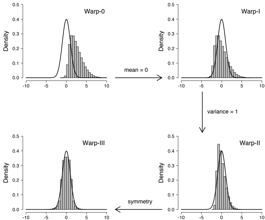
Figure 2: Illustration of the warping procedure. The black solid line shows the standard normal proposal distribution and the gray histogram shows the posterior samples. Figure also available at https://tinyurl.com/y7owvsz3 ; see also Gronau et al. 2020a, 2019).
