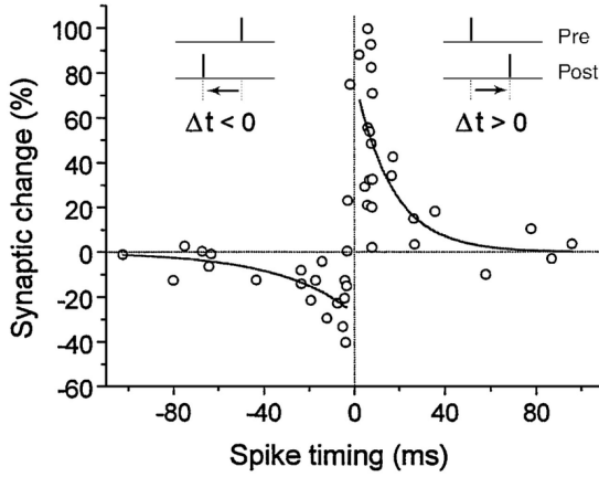
Figure 6.1.: The STDP learning rule (figure from Bi and Wang [2002]), showing the Synaptic change \Delta w_{ij} on the y-axis, as a function of the relative timing between the pre and post-synaptic spikes \Delta t = t_{post} - t_{pre} on the x-axis. The anti-symmetrical double-exponential curve very roughly models data from neural recordings (points)
