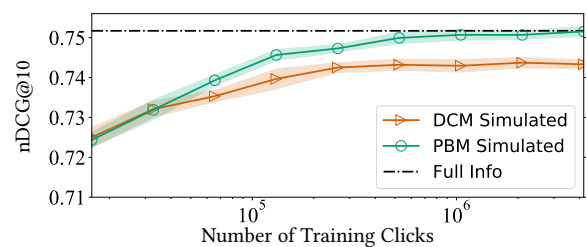
Figure 1: Performance of PBM-IPS CLTR on different sets of simulated clicks.
