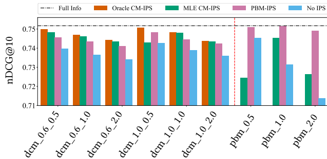
Figure 2: Performance of PBM-IPS and CM-IPS CLTR on different sets of simulated clicks. We repeated each experiment 15 times and report the mean value.
