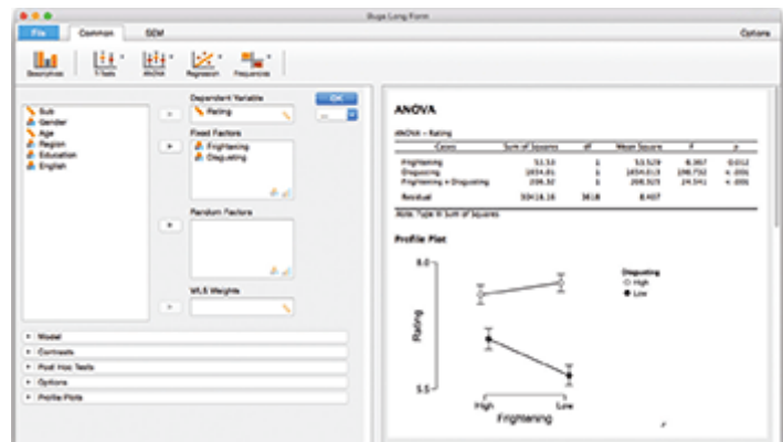
Figure 1. JASP screenshot of an ANOVA performed on a subset of “bugs” data from Ryan, Wilde, and Crist (2013) concerning repulsiveness ratings for sets of frightening and/or disgusting insects.
