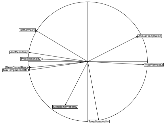
correlation circle
