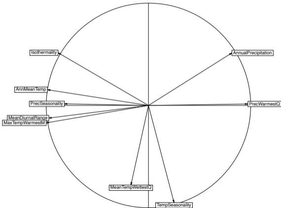
correlation circle
