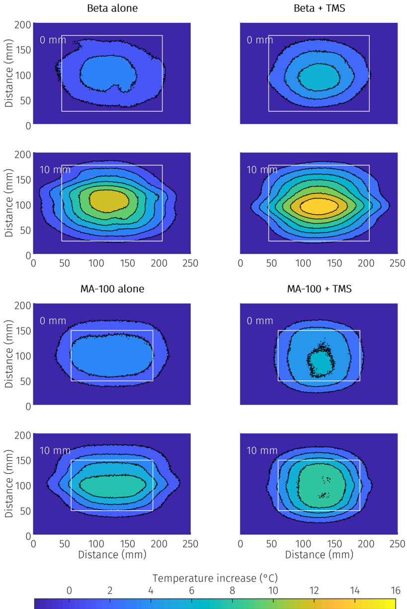
Figure 7. The infrared temperature data of the power deposition pattern of the Beta (51.0 W at 434 MHz; Medlogix, Rome, Italy) and MA-100 (44.1 W at 915 MHz; Pyrexar, Salt Lake City, USA) applicators. The temperature rise on the surface of the fat-equivalent layer is shown (0 mm) and at 10 mm depth on the surface of the muscle-equivalent phantom (10 mm). Results are displayed for the applicator alone (left) and the applicator combined with the thermal monitoring sheet (TMS; right). The aperture dimensions are represented by the white rectangle.
