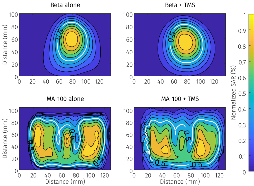
Figure 8. Normalized SAR distribution of the Beta and MA-100 applicators alone (left) and the applicators combined with the thermal monitoring sheet (TMS; right) at 10 mm depth in a liquid muscle-equivalent phantom. The effective field of the applicators is depicted in white.
