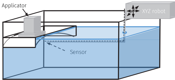
Figure 5. E-field probe measurements of the power deposition patterns were performed in a 1000 x 400 x 400 mm Plexiglas tank, filled with 80 L muscle-equivalent saline solution (0.6 % NaCl). To mount the applicator in the tank, a Plexiglas mounting box with similar curvature as the phantom in Figure 4 was submerged in the larger Plexiglas tank. The E-field was automatically scanned using an E-field sensor (20 mm in-house built diode dipole with high resistance leads) attached to an in-house built positioning system (resolution 0.1 mm; XYZ robot assembled from parts from Igus, Cologne, Germany) in a 2.9 x 2.0 mm (X x Y) grid at 10 mm depth.
