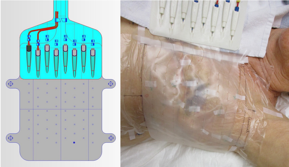
Figure 2. The left picture is a schematic drawing of the thermal monitoring sheet (TMS; Medlogix, Rome, Italy). Dimensions of the transparent silicone sheet are 212.5 x 166 x 0.3 mm (lxwxh) with eight seven-sensor thermocouple probes resulting in a monitoring area of 162.5 x 140 mm. The right picture shows a photograph of the TMS on the chest wall of a study patient.
