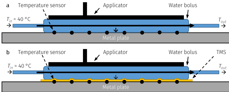
Figure 6. Experimental set-up to determine the heat transfer of (a) the water bolus alone, and (b) the water bolus with the thermal monitoring sheet (TMS).
