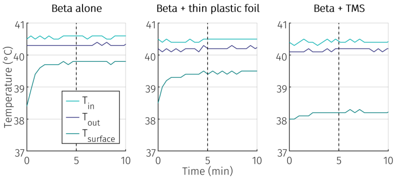
Figure 9. The effect of the 10 \mu\text{m} high density polyethylene plastic foil and TMS on the heat transfer of the water bolus of the Beta applicator. The five minute steady state interval starts after the dotted vertical line. The median temperature of the inflow ( T_{in} ), outflow ( T_{out} ) and the median surface temperature ( T_{surface} ) are presented during a ten minute interval.
