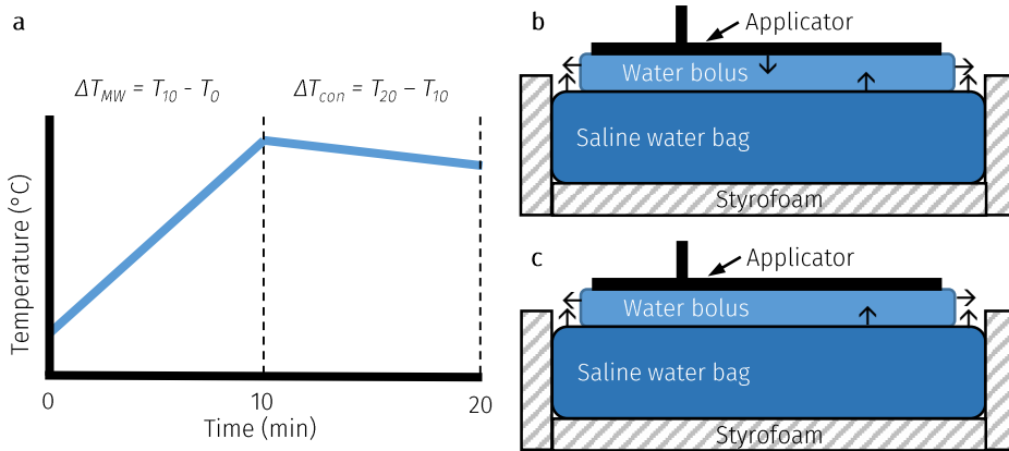
Figure 3. The experimental set-up to determine the applicator efficiency. (a) Power was applied for ten minutes to the saline water bag which causes a temperature increase ( \Delta T_{MW} ), after turning off power the temperature decline due to conductive heat transport was measured for ten minutes ( \Delta T_{con} ) to arrive at an estimate for the heat loss to the environment during heating (equation 2). (b) The heat transport during the heat up phase and (c) cool down phase are depicted with black arrows.
