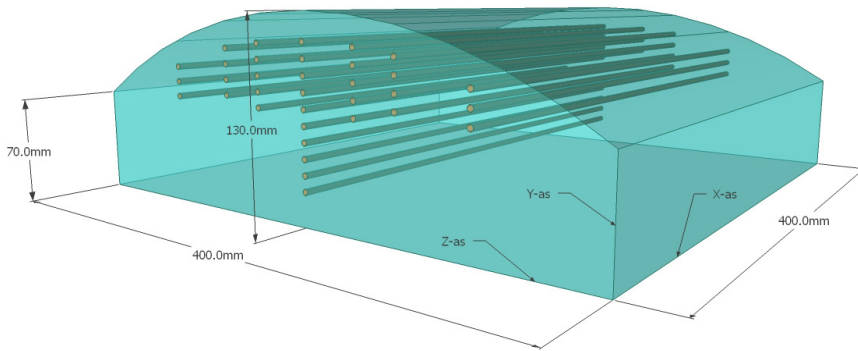
Figure 4. The slightly curved muscle-equivalent phantom used in the experiment to evaluate the power distribution pattern with the infrared (IR) camera. Catheters are positioned inside the phantom for invasive thermometry. The 10 mm thick fat-equivalent layer that can be positioned on top is not depicted. IR images are taken of the surface of the muscle-equivalent phantom and the 10 mm fat-equivalent layer.
