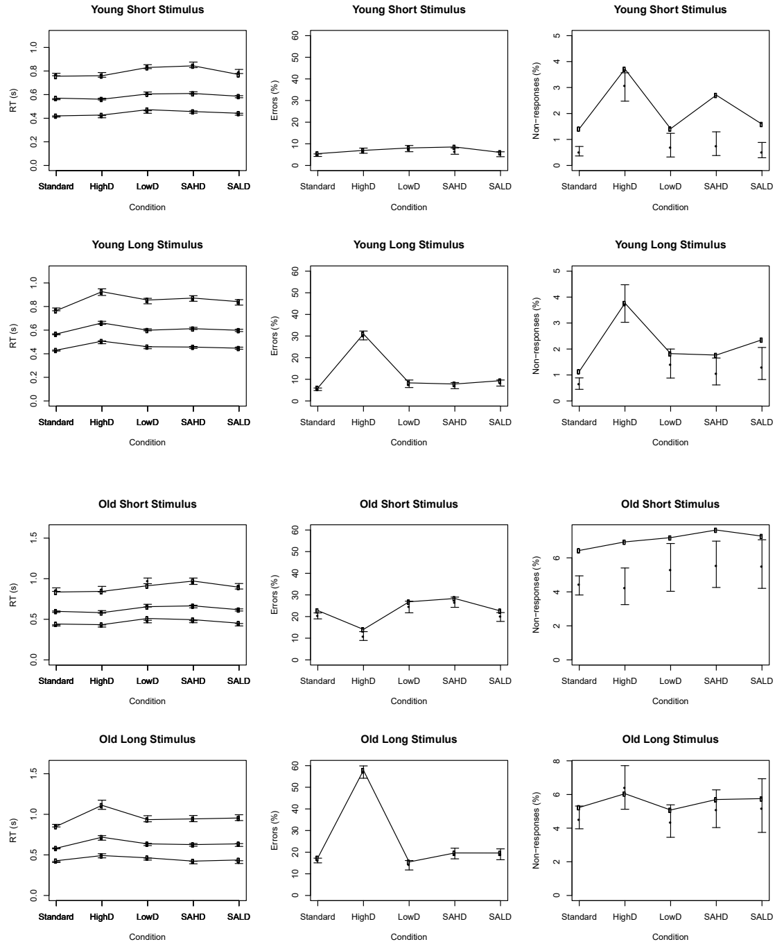
Figure 3. Fit of the most flexible intrinsic and contaminant model in Table 2. The three lines in the left column are the 10 th , 50 th and 90 th percentiles of RT distributions. Data are open circles joined by lines. Fits are shown with 95% credible intervals. HighD = High Deviant, LowD = Low Deviant, SAHD = Standard After High Deviant, SALD = standard after low deviant.
