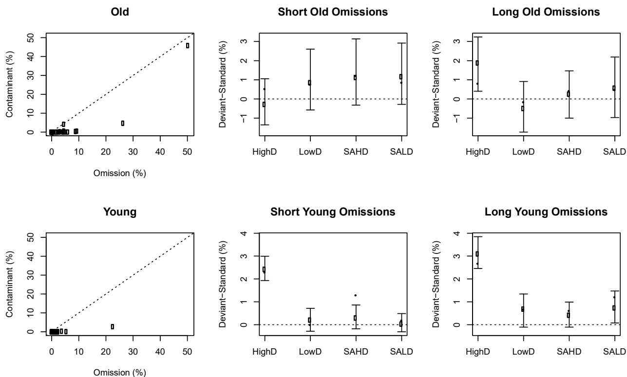
Figure 4. Parameters and fit of the most flexible intrinsic and contaminant model in Table 2. The left column shows individual participant omission percentages against the posterior median of the contaminant omission parameters estimated by the model. The middle and right columns show differences between the standard and deviant conditions omission percentages for the data (solid symbols) and the model (open symbols with 95% credible intervals). HighD = High Deviant, LowD = Low Deviant, SAHD = Standard After High Deviant, SALD = standard after low deviant.
