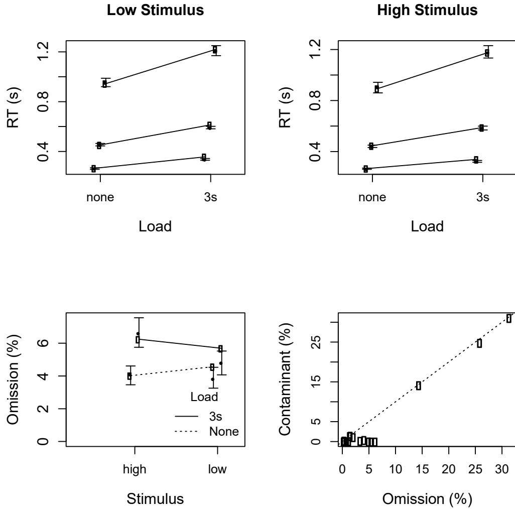
Figure 1. Top row: RT distributions (lower, middle, and upper lines and points are 10 th , 50 th , and 90 th percentiles, respectively). Bottom left panel: Omission percentages data (open symbols), with model fits of the selected model in Table 1 as posterior predictive medians (solid points) and 95% credible intervals. Bottom right panel: Individual participant omission percentages against the posterior median of the contaminant omission parameters estimated by the model. Load conditions: none and 3s (i.e., count backwards by 3s).
