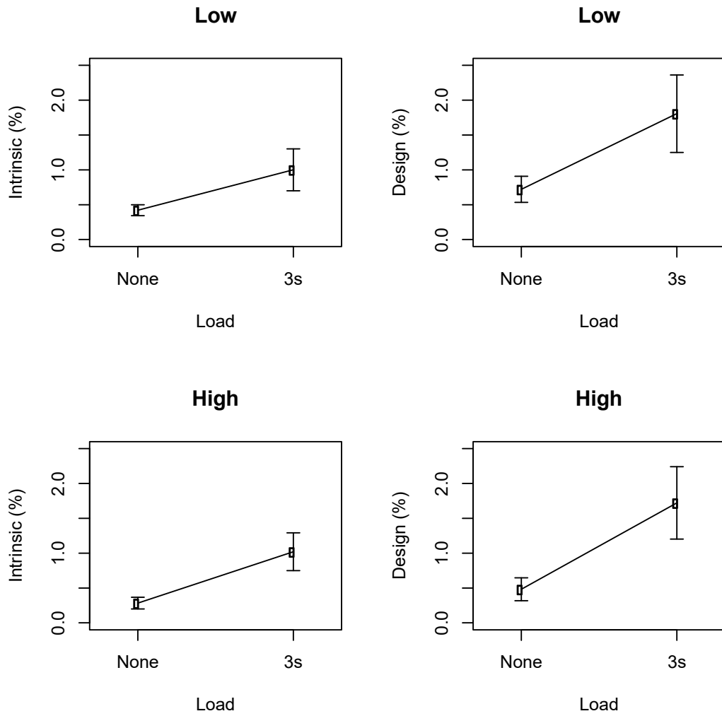
Figure 2. Median and 95% credible intervals for the posterior predictive distribution of process omissions computed for the model selected in Table 1. The left column displays intrinsic omissions and the right column design omissions with the upper row containing results for low stimulus and the lower row for high stimuli.
