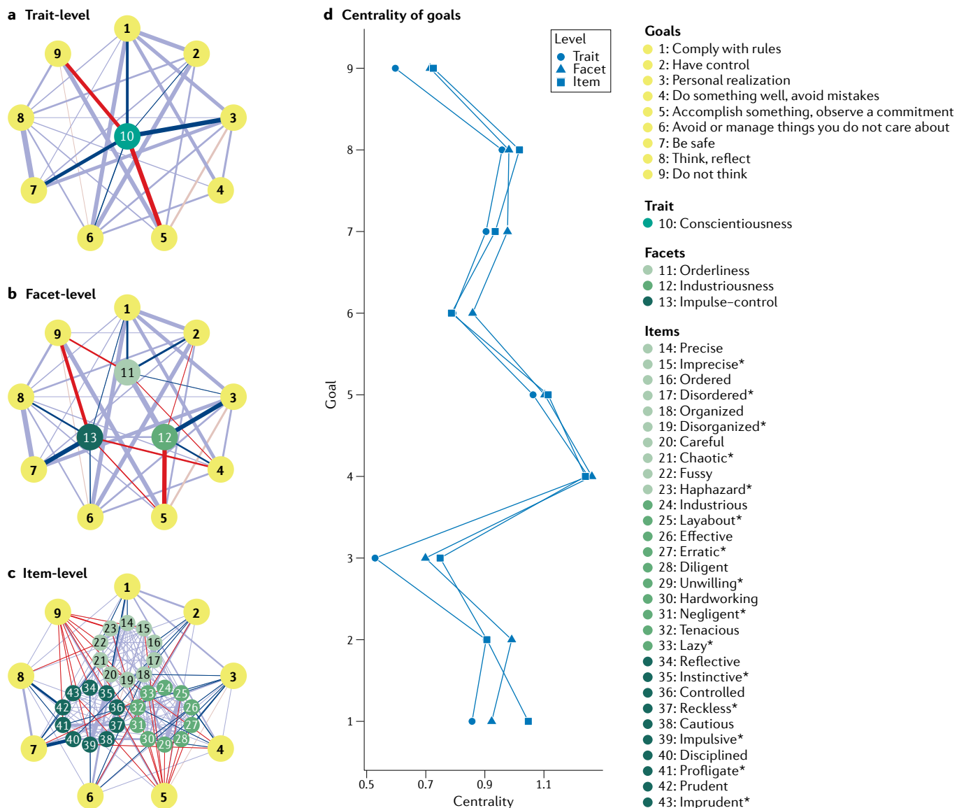
Fig. 4 | Strength centrality estimates for all nodes in three networks of personality research data.
