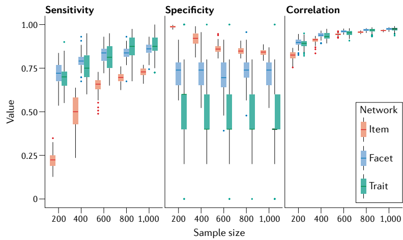
Fig. 8 | Projected replicability for the personality network as assessed through the ReplicationSimulator function in the bootnet R package.
