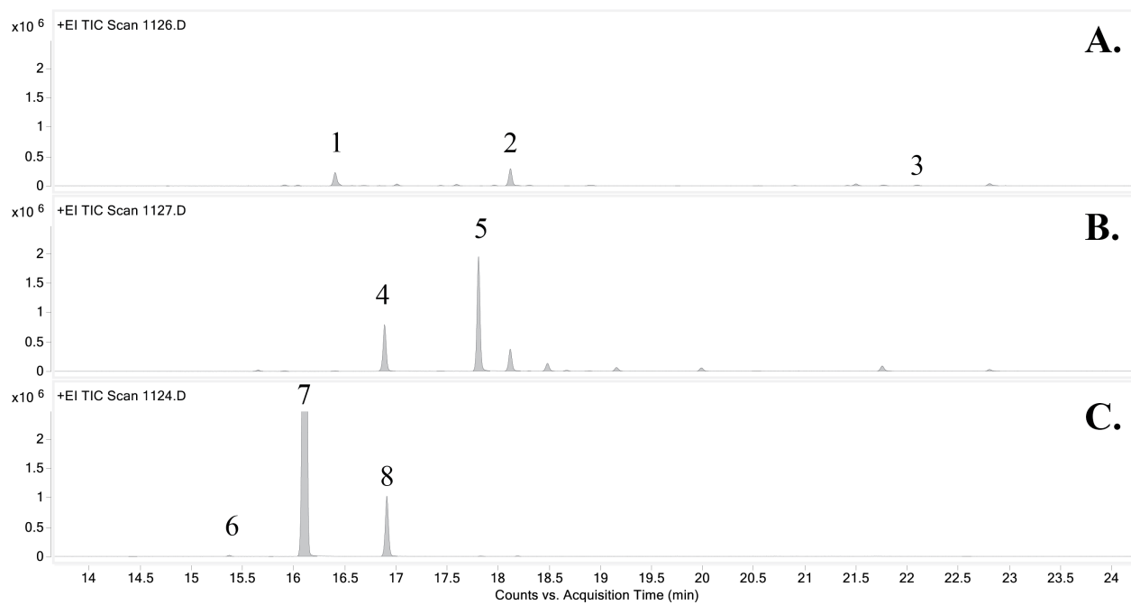
Figure S5: Citrus bergamia STS chromatograms Chromatograms obtained from the R. sphaeroides strain expressing A. MT636927, B. MT636928, and C. MW384854 with peaks labelled.
