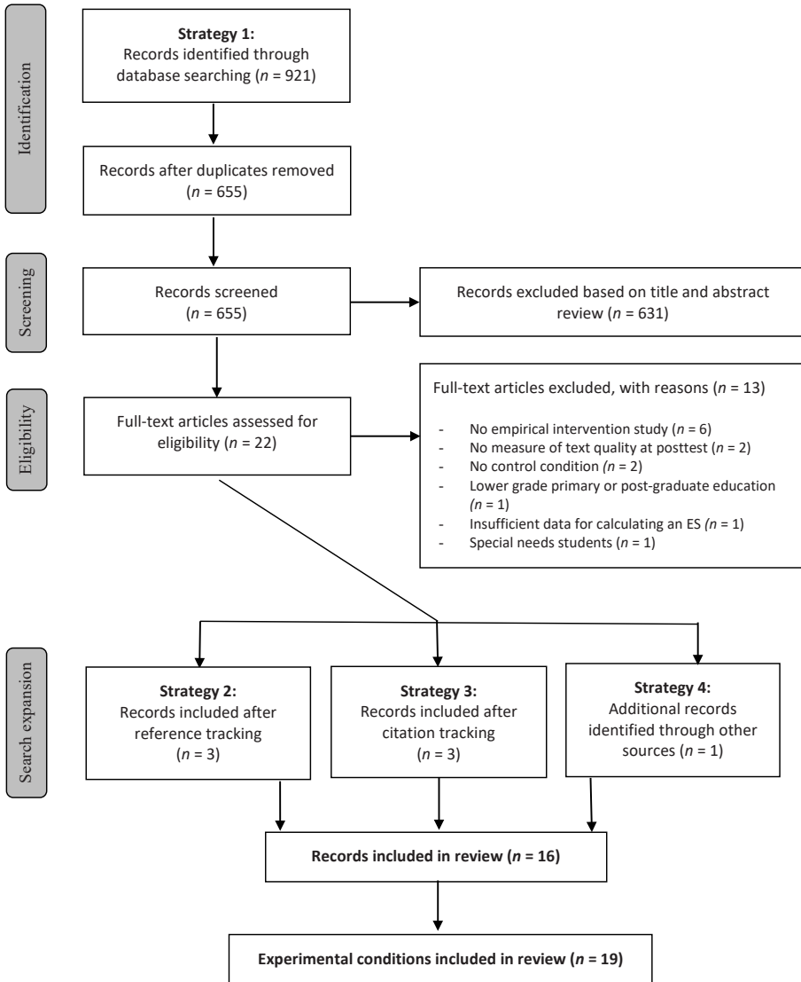
Figure 2.1 Flow chart of the literature selection procedure.
