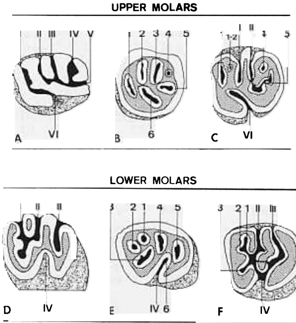
Fig. 2. Comparison of occlusal patterns in different stages of wear of upper and lower cheek-teeth of Hystrix (A, B, D, E) and Trichys (C, F) specimens. Upper molars: A = M1 of H. brachyura (ZMA 1270) with folds I - VI, B = M2 of H. brachyura (ZMA 6855) with islands 1 - 6, C = M1 of Trichys fasciculata (ZRC 4.1622) with folds and islands. Lower molars: D = m3 of H. brachyura (ZMA 6870) with folds I - IV, E = m2 of H. brachyura (ZMA 1128) with islands 1 - 5 and fold VI, and F = m1 of Trichys fasciculata (ZRC 4.1622) with folds and potential islands. All molars are left ones and not figured to the same scale. Indication of folds and islands after Van Weers (1990).
