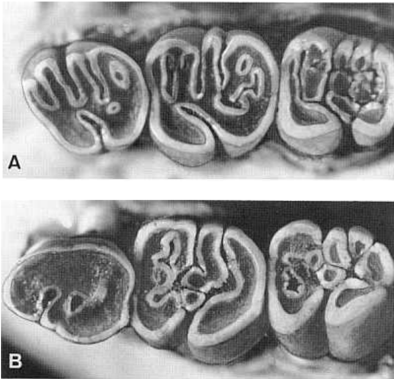
Fig. 4. Left D4 - M2 (A) and d4 - m2 (B) of Trichys fasciculata , specimen ZRCS 4.1622 from Mt. Kinabalu, Borneo. Protocone respectively protoconid directed to the bottom of the page, figures \pm x7 .
