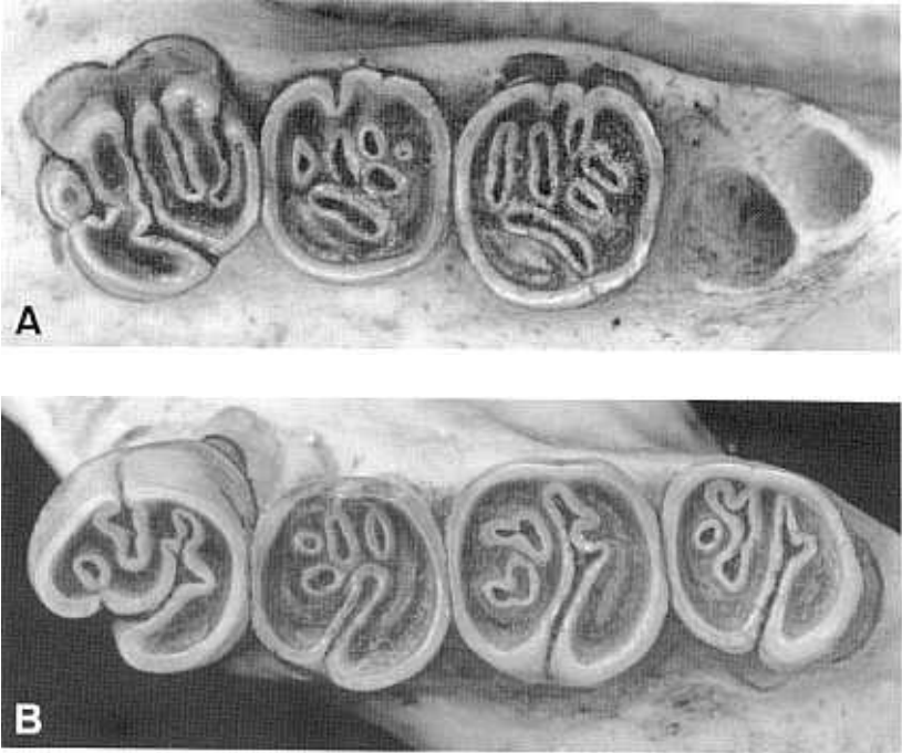
Fig. 3. Left P4 - M2 (A) and p4 - m3 (B) figured as a left one, Trichys fasciculata , specimen ZMA 22.224 from Sarawak, Borneo. Protocone, respectively protoconid directed to the bottom of the page, figures \pm x7 .
