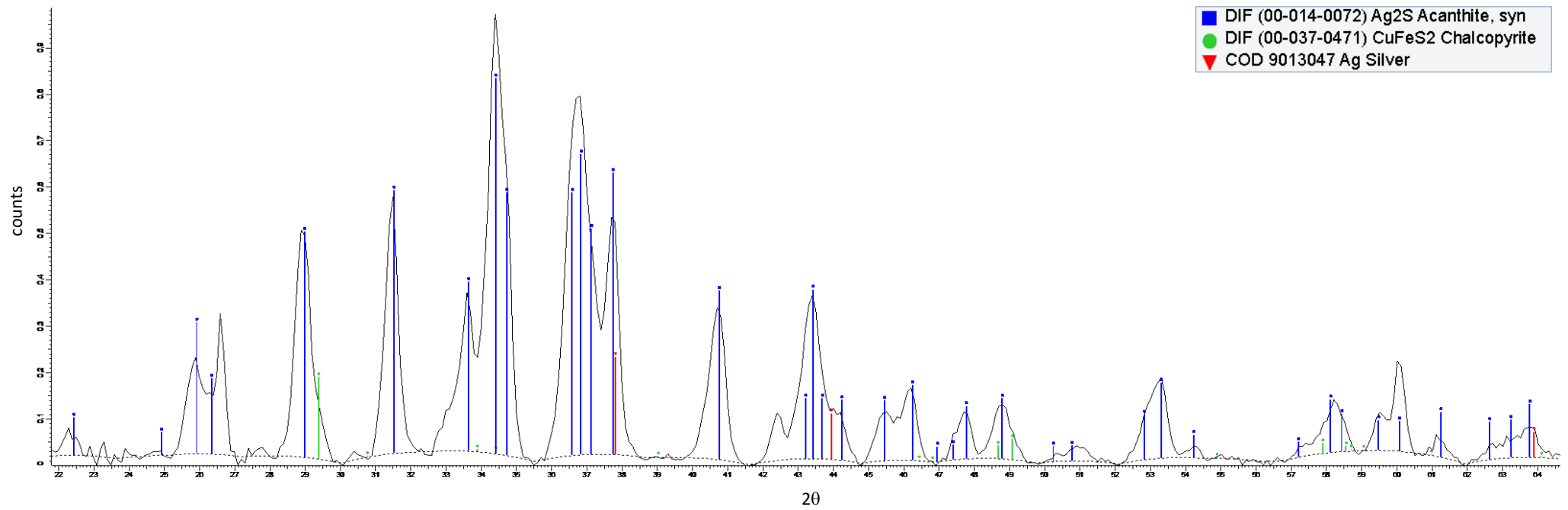
Fig. AF5: Powder that has fallen off from sphere 5372-122 during handling. Diffractogram after background subtraction.
