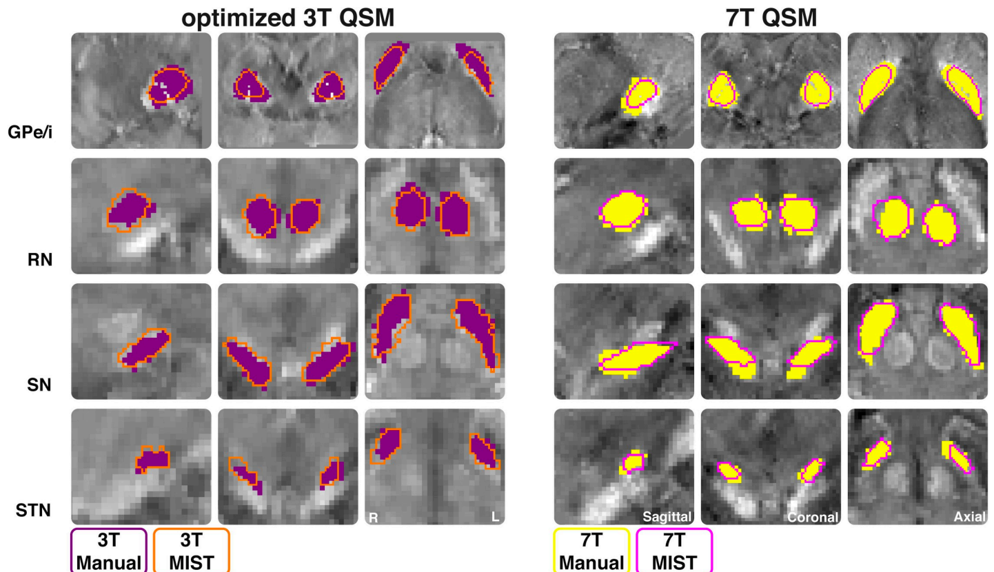
Fig 4. MIST parcellations. Outline of masks for each structure manually parcellated optimized 3T (o3T) (left) and 7T (right) from a single subject. Manual masks are shown in opaque purple for o3T and yellow for 7T. MIST masks are shown as an orange outline for o3T and pink outline for 7T. Structures are shown in the coronal, sagittal, and axial planes. QSM contrasts were used for all parcellations. QSM = quantitative susceptibility mapping, GPe/i = combined globus pallidus externa and interna, RN = red nucleus, SN = substantia nigra, STN = subthalamic nucleus.
