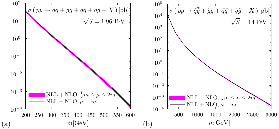
Figure 6. The NLL+NLO cross section for inclusive squark and gluino pair-production, p\bar{p}/pp \rightarrow \tilde{q}\bar{\tilde{q}} + \tilde{g}\bar{\tilde{g}} + \tilde{q}\bar{\tilde{q}} + \tilde{g}\bar{\tilde{g}} + X , at the Tevatron (a) and the LHC (b) as a function of the average sparticle mass m . Shown are results for the mass ratio r = m_{\tilde{g}}/m_{\tilde{q}} = 1 . The error band corresponds to a variation of the common renormalization and factorization scale in the range m/2 \leq \mu \leq 2m .
