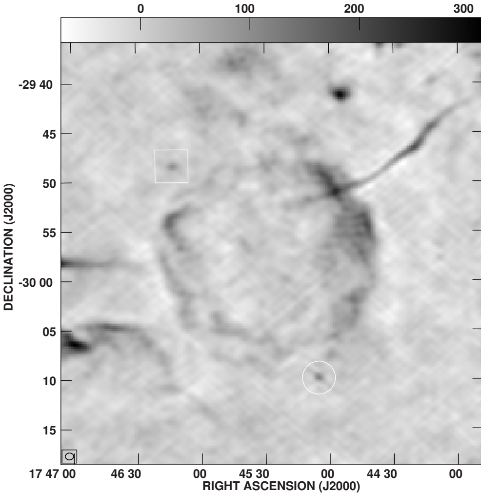
Figure 4.1: The supernova remnant G359.1-0.5 with "The Snake" to the northwest, from our reduction of the GCRT J1745-3009 discovery observation on 2002 September 30/October 1 with the VLA in CnB configuration. This observation revealed this transient, indicated by a circle, for the first time (see Hyman et al. 2005). Noise levels in this image vary from 5 to 13 mJy beam -1 across the image. A Gaussian fit to the unresolved GCRT J1745-3009 gives a peak flux density of only 116 \pm 14 mJy beam -1 because the five Jy-level bursts have been averaged over about 6h of observation. A Gaussian fit to the source to the northeast of the supernova remnant, indicated by the box, gives a peak flux density of 91 \pm 14 mJy beam -1 . Correction for primary beam attenuation has been applied.
