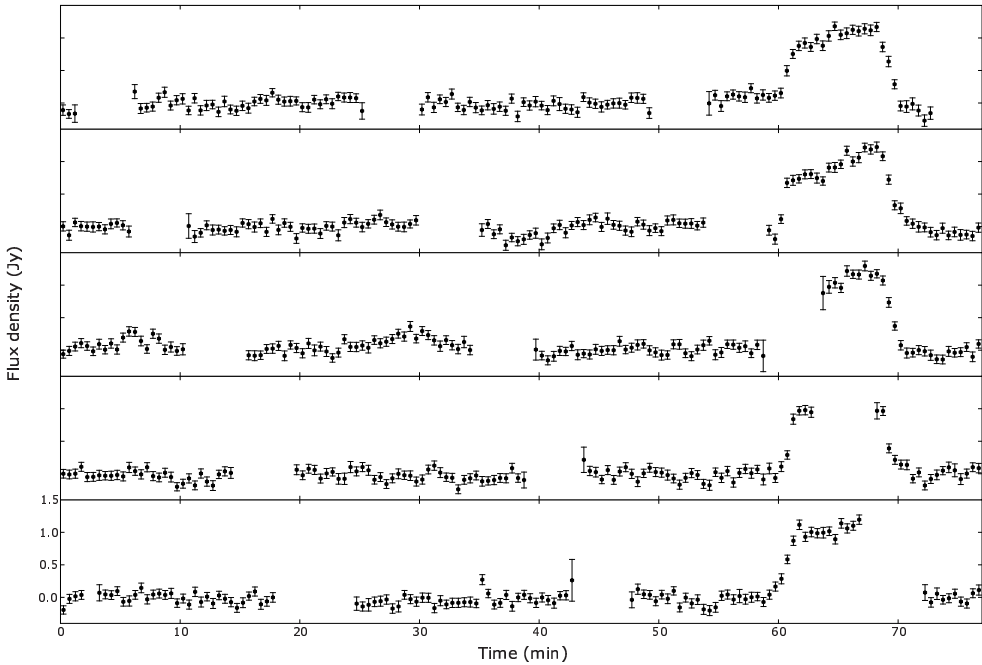
Figure 4.3: The plot above shows the lightcurve from the discovery dataset of GCRT J1745-3009 with 30s sampling. This plot is setup in the same way as the lightcurve in the discovery paper except for the flux density measurements between bursts. For those nondetections Hyman et al. (2005) showed 3\sigma upper limits on interburst emission, we show the actual background flux density measurements. Also, we have folded the lightcurve at intervals of 77.012 minutes instead of 77.130 minutes. The first interval is shown in the bottom panel, starting at 20h50m00s on 2002 September 30 (IAT). The average of all the error bars shown is 74 mJy. The gaps are due to phase calibrator observations.
