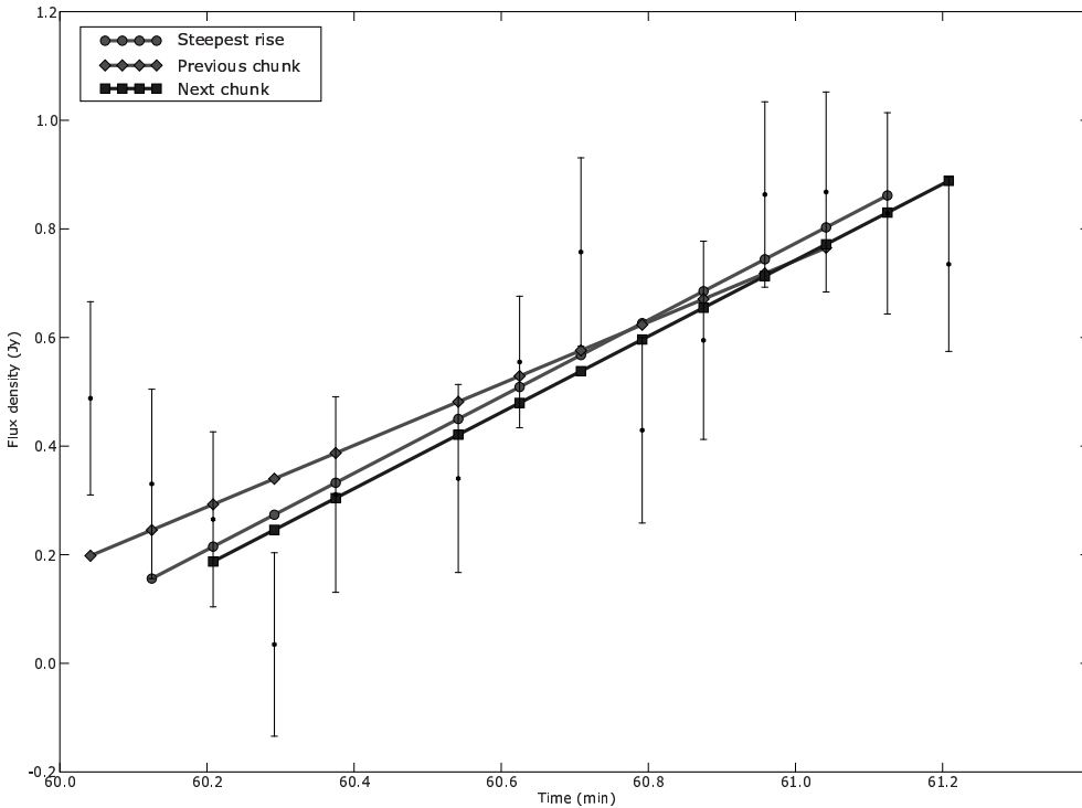
Figure 4.4: This plot illustrates how the times of steepest rise for four of the bursts are determined. Weighted linear regression is performed on successive one minute chunks of data. The chunks have a maximum of 55s of overlap time. Here the rising part of the first burst is shown.
