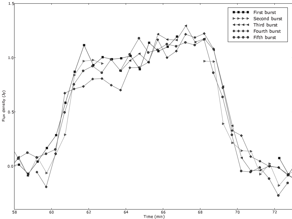
Figure 4.5: The plot above shows the five bursts from the discovery dataset of GCRT J1745-3009 with 30s sampling folded at intervals of 77.012 minutes. Time is relative to 20h50m00s on 2002 September 30 (IAT) (plus multiples of 77.012 minutes).
