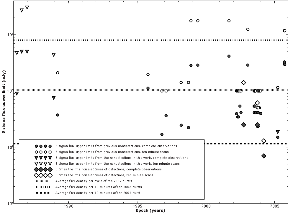
Figure 4.2: Approximate detection thresholds ( 5\sigma noise levels) at the location of GCRT J1745-3009 of 41 Galactic Center observations at 92 cm over two decades. For the WSRT observation at 92 cm, the 10 minute scan sensitivity is not indicated, since the snapshot point spread function (psf) of a linear array does not allow to do this accurately. The observations in this plot start on 1986 March 29 and end on 2005 September 27.
