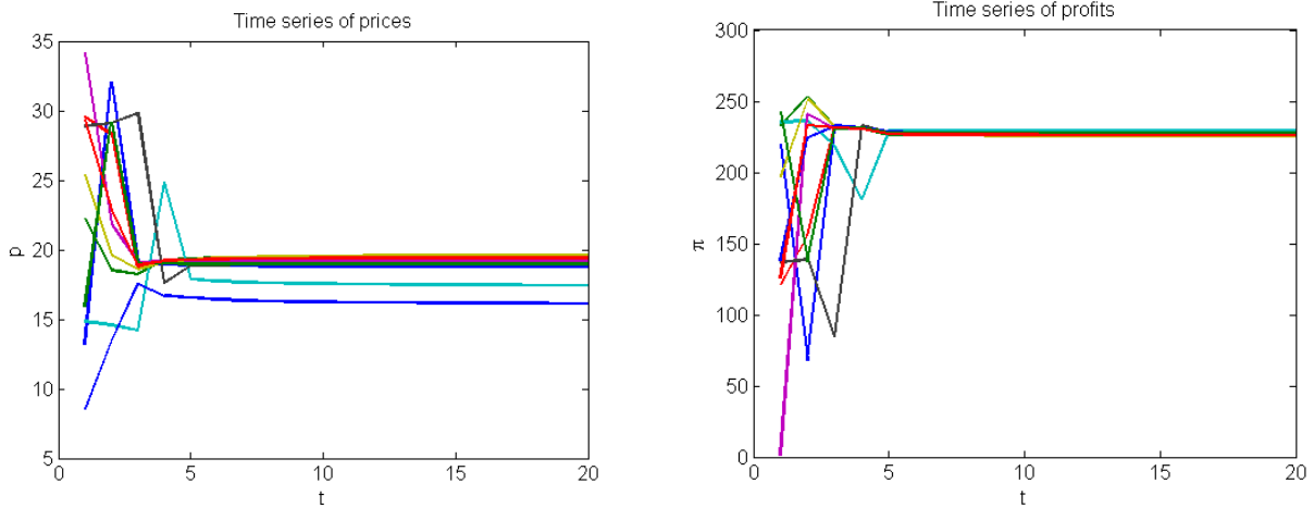
Figure 3: Time series of prices (left) and profits (right) in an oligopoly with 10 OLS learners. Parameter values: \alpha_1 = 35 , \alpha_2 = 4 , \alpha_3 = 2 , \beta = 0.7 , \gamma = 0.6 , c = 4 and \delta = 10^{-8} . Nash equilibrium values: p_N \approx 17.7693 and \pi_N \approx 223.9148 .
