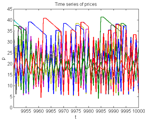
(c) Aperiodic dynamics for \lambda = 1
