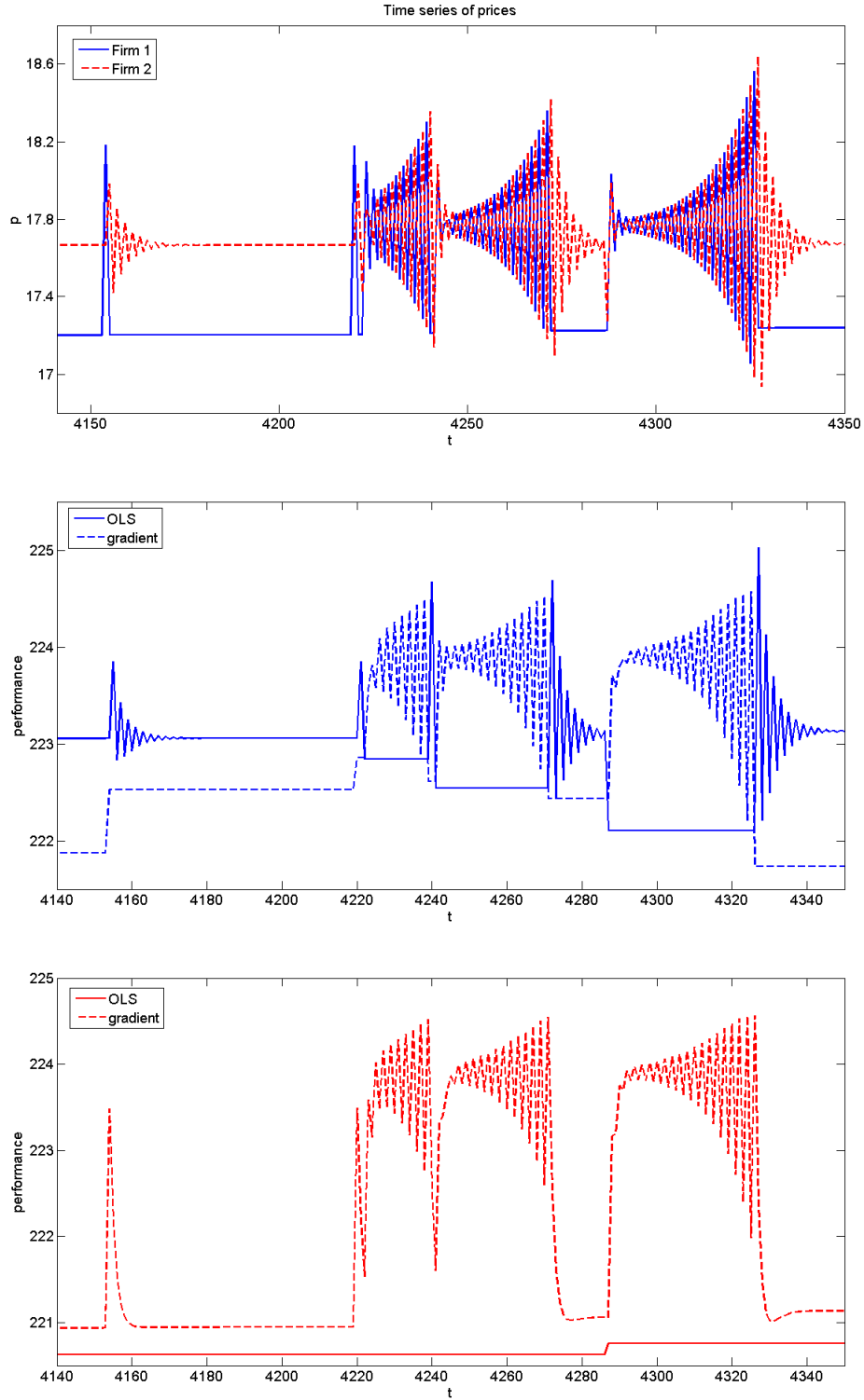
Figure 8: Cyclical switching in a duopoly. Time series of prices (upper panel), the performance measures of firm 1 (middle panel) and firm 2 (lower panel). Parameter values: \alpha_1 = 35 , \alpha_2 = 4 , \alpha_3 = 2 , \beta = 0.7 , \gamma = 0.6 , c = 4 , \lambda = \lambda_0 = 0.85 and k = 1 .
