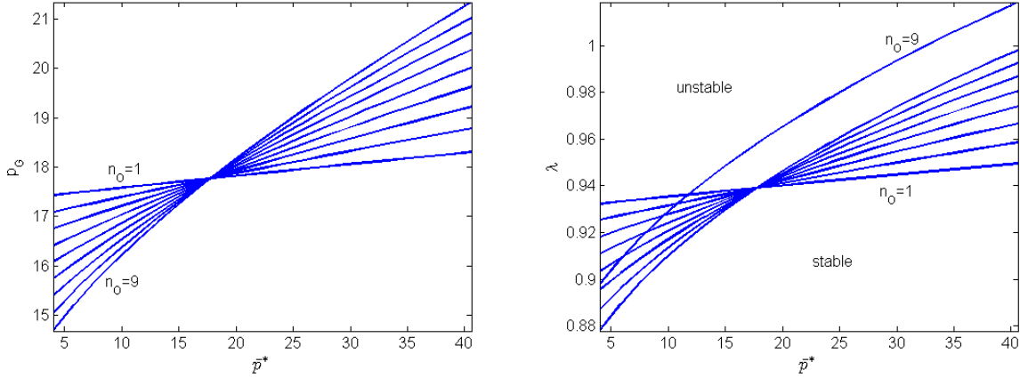
Figure 5: The gradient learners’ price (left panel) and the stability-instability region for different number of OLS learners. Parameter values: \alpha_1 = 35 , \alpha_2 = 4 , \alpha_3 = 2 , \beta = 0.7 , \gamma = 0.6 and c = 4 .
