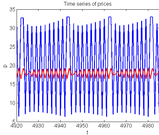
(b) Quasi-periodic dynamics for \lambda = 0.9344
