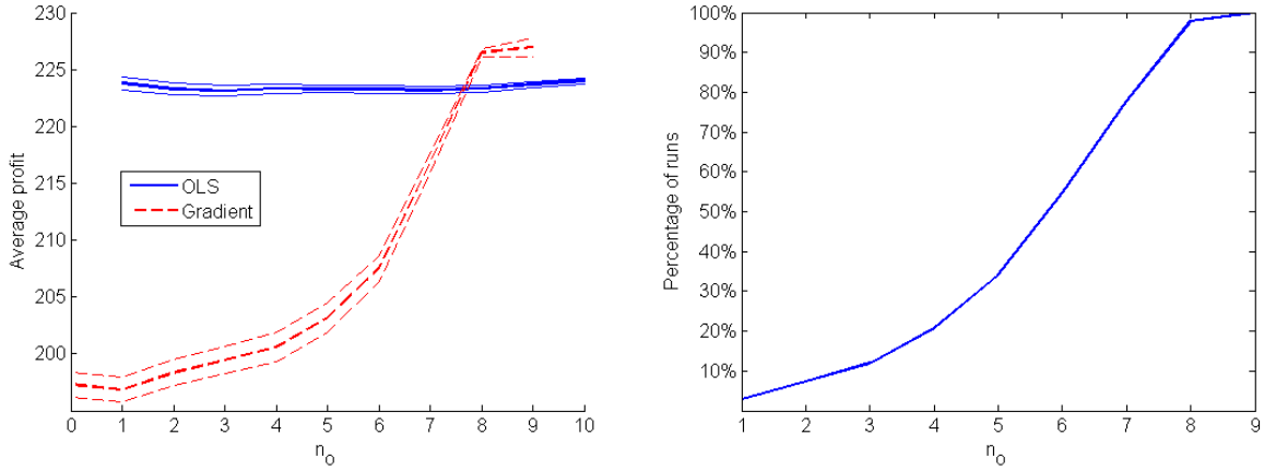
Figure 7: The average OLS and gradient profits (with 95% confidence interval) (left panel) and the percentage of runs in which gradient learners earn a higher average profit. Parameter values: \alpha_1 = 35 , \alpha_2 = 4 , \alpha_3 = 2 , \beta = 0.7 , \gamma = 0.6 , c = 4 and \lambda = \lambda_0 = 0.937 .
