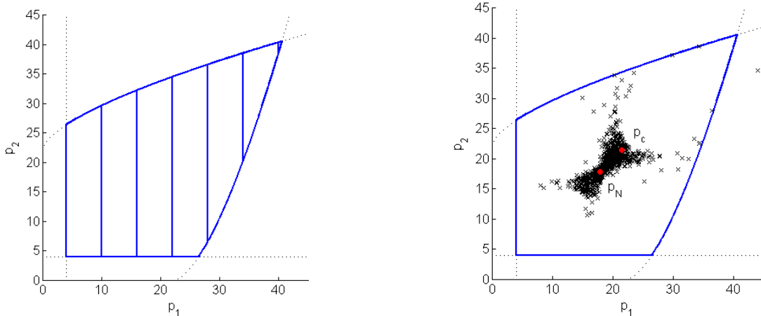
Figure 2: The set of SSE prices for two firms (left panel) and the end prices of simulations with initial prices drawn from the uniform distribution on the set of SSE prices (right panel). Parameter values: \alpha_1 = 35 , \alpha_2 = 4 , \alpha_3 = 2 , \beta = 0.7 , \gamma = 0.6 , c = 4 and \delta = 10^{-8} .
