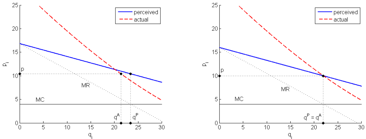
Figure 1: Disequilibrium (left) and self-sustaining equilibrium (right) of the model with OLS learning. Parameter values: \alpha_1 = 35 , \alpha_2 = 4 , \alpha_3 = 2 , \beta = 0.7 , \gamma = 0.6 , c = 4 and \bar{p}_{-i} = 8 .
