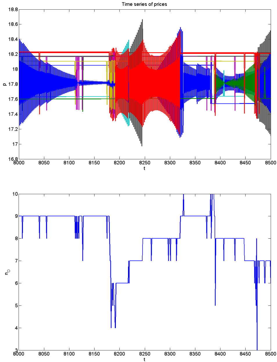
Figure 9: Cyclical switching with 10 firms. Time series of prices (upper panel) and number of OLS learners (lower panel). Parameter values: \alpha_1 = 35 , \alpha_2 = 4 , \alpha_3 = 2 , \beta = 0.7 , \gamma = 0.6 , c = 4 , \lambda = \lambda_0 = 0.95 and k = 5 .
