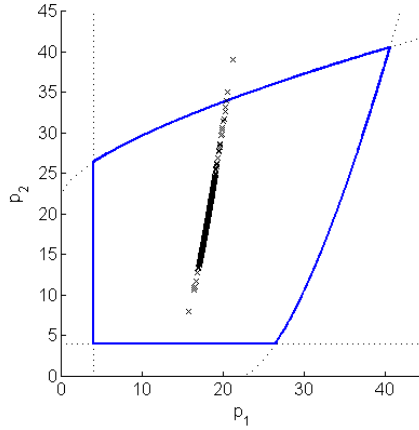
Figure 6: The end points of the simulations with firm 1 as gradient learner and firm 2 as OLS learner. Parameter values: \alpha_1 = 35 , \alpha_2 = 4 , \alpha_3 = 2 , \beta = 0.7 , \gamma = 0.6 , c = 4 , \lambda = \lambda_0 = 0.5 and \delta = 10^{-8} .
