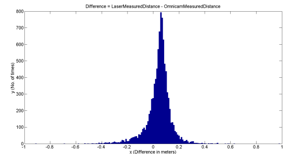
(b) Factory: Histogram of the omnica accuracy
