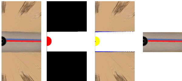
(a) Bird-eye view image of the factory environment. (b) Laser range measurements image. (c) Image created by the combined bird-eye view image and the laser image. (d) The resulting image that is used for training.
