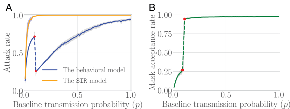
Fig. 2. Dueling dynamics of the behavioral model. (A) Contrasting the behavioral model with the SIR model. Shown is the attack rate as a function of the disease baseline transmission probability ( p ) for the behavioral model (blue line) and for the SIR model (orange line). (B) Social dynamics of the behavioral model. Shown is the mask acceptance rate as a function of p . The variances are shown as shaded regions, with one SD above and below the mean. The two tipping points for the behavioral model are highlighted in red. All parameters are set to their baseline values shown in Table 1.
