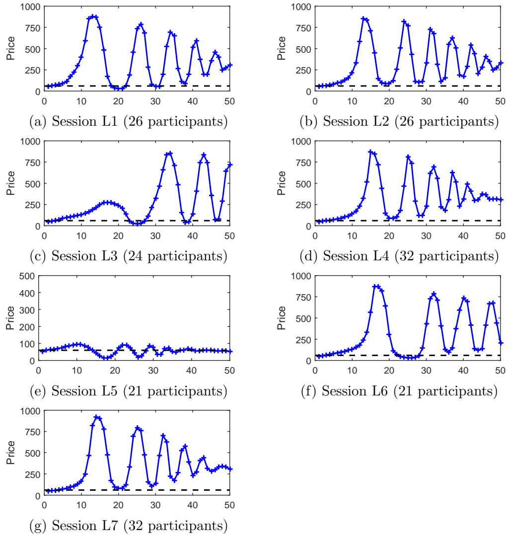
Figure 4: Realized market prices The dashed line indicates the fundamental value of 60. Note that the vertical axis for session L5 runs up to 500 instead of 1000.
