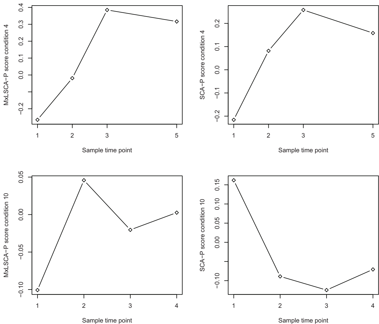
Figure 3 Scores on the third component of MxLSCA-P and SCA-P. Scores on the third component of MxLSCA-P (left) and SCA-P (right) for experimental conditions 4 and 10 (from top to bottom the first and second row of panels, respectively). On the x-axis, the different time points of sampling are presented ranging from 'early' (1) to 'late' (3, 4, and 5). The y-axis indicates the score value in arbitrary units.
